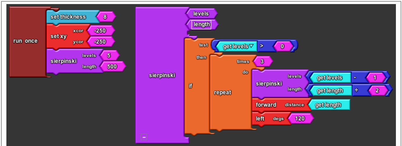
a. A TurtleBlocks program for drawing Sierpinski's gasket.
