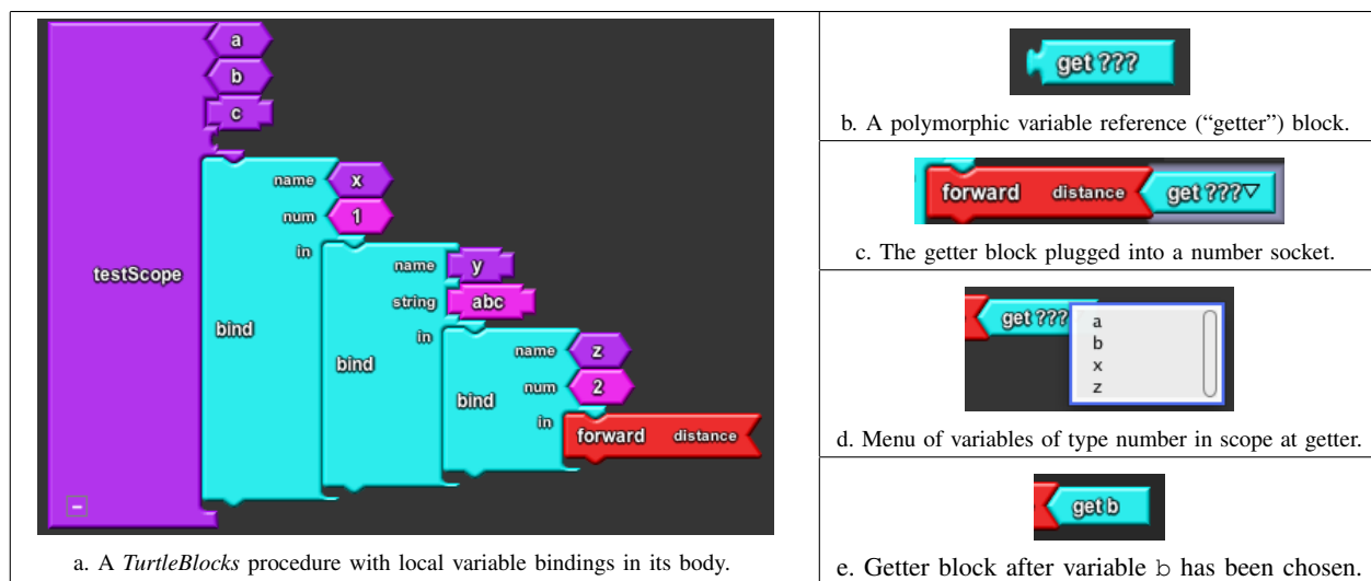
Fig. 12. An illustration of variable scope in TurtleBlocks .
