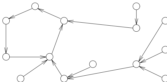
Figure 3.7: A pseudotree.
