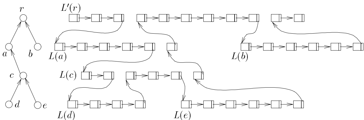
Figure 3.14: The effect of the plugging step execution by all vertices of a pseudotree but the representative r . On the left is P = (C, D) . On the right is L'(r) after the execution of the plugging step.
