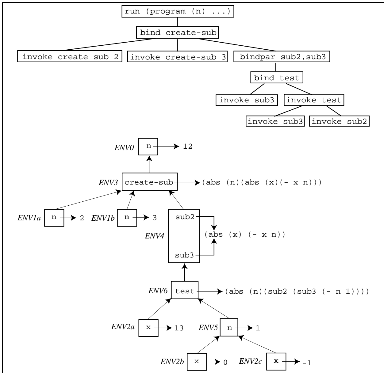
Figure 2: Invocation tree and environment diagram for the create-sub program run on 12.
