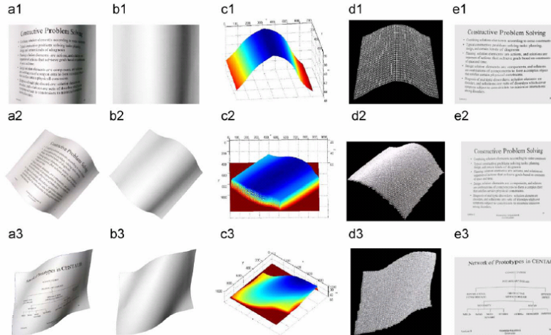
Fig. 16. (a 1 ), (a 2 ), (a 3 ) Distorted real document images; (b 1 ), (b 2 ), (b 3 ) extracted shading image; (c 1 ), (c 2 ), (c 3 ) reconstructed surface shape; (d 1 ), (d 2 ), (d 3 ) the 3D mesh of the surface shape and (e 1 ), (e 2 ), (e 3 ) final restored image with all the distortions removed.
