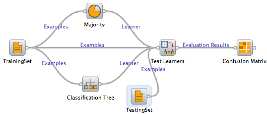
Figure 3: Comparing the classification results between a tree classifier and the majority classifier.
