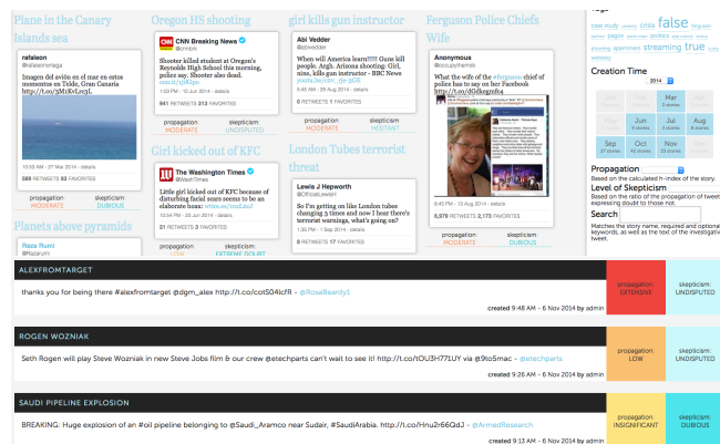
Figure 3: The full story view page (top) and condensed view page (bottom) of twittertrails.com .
