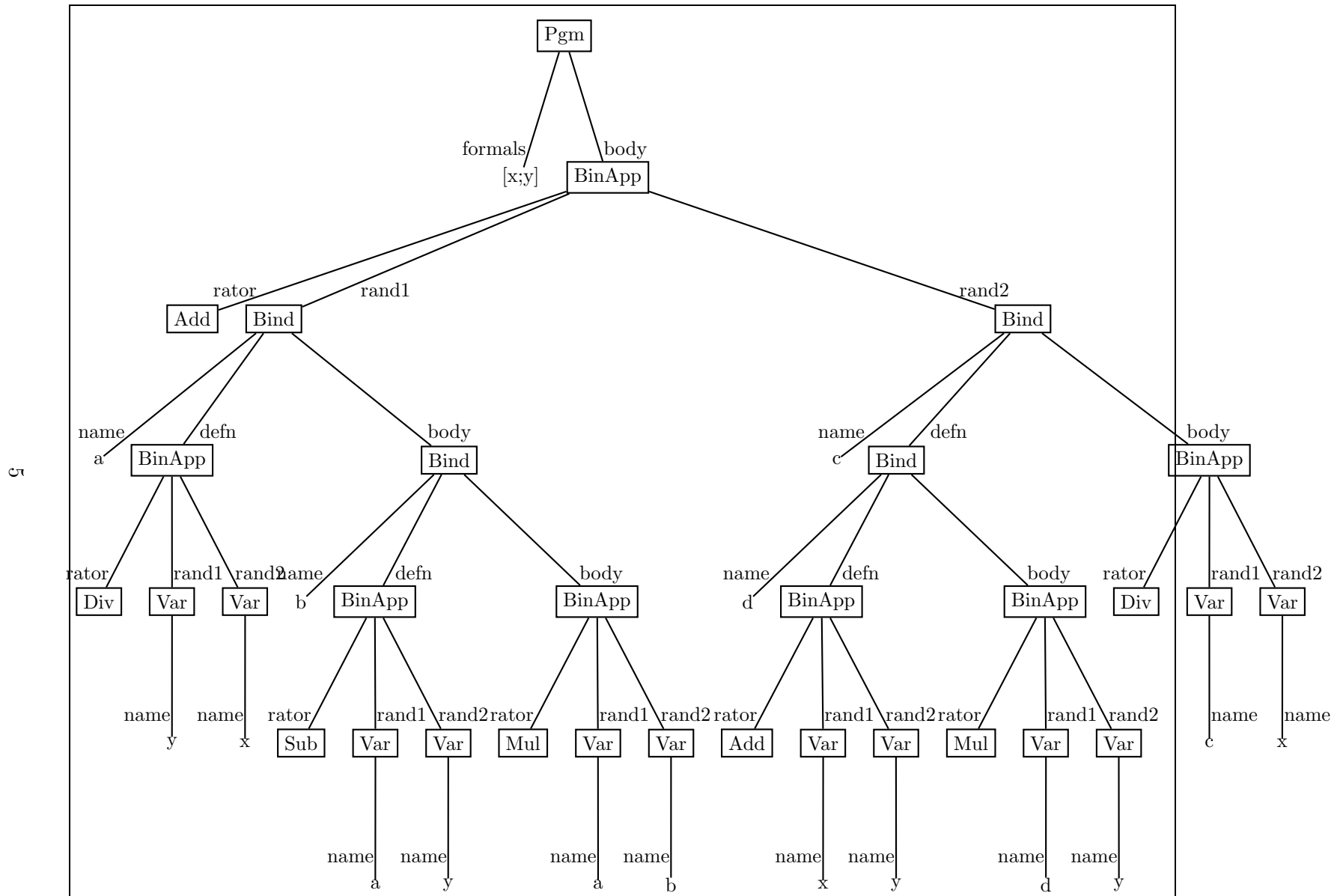
Figure 2: Abstract syntax trees for the sample BINDE program.
